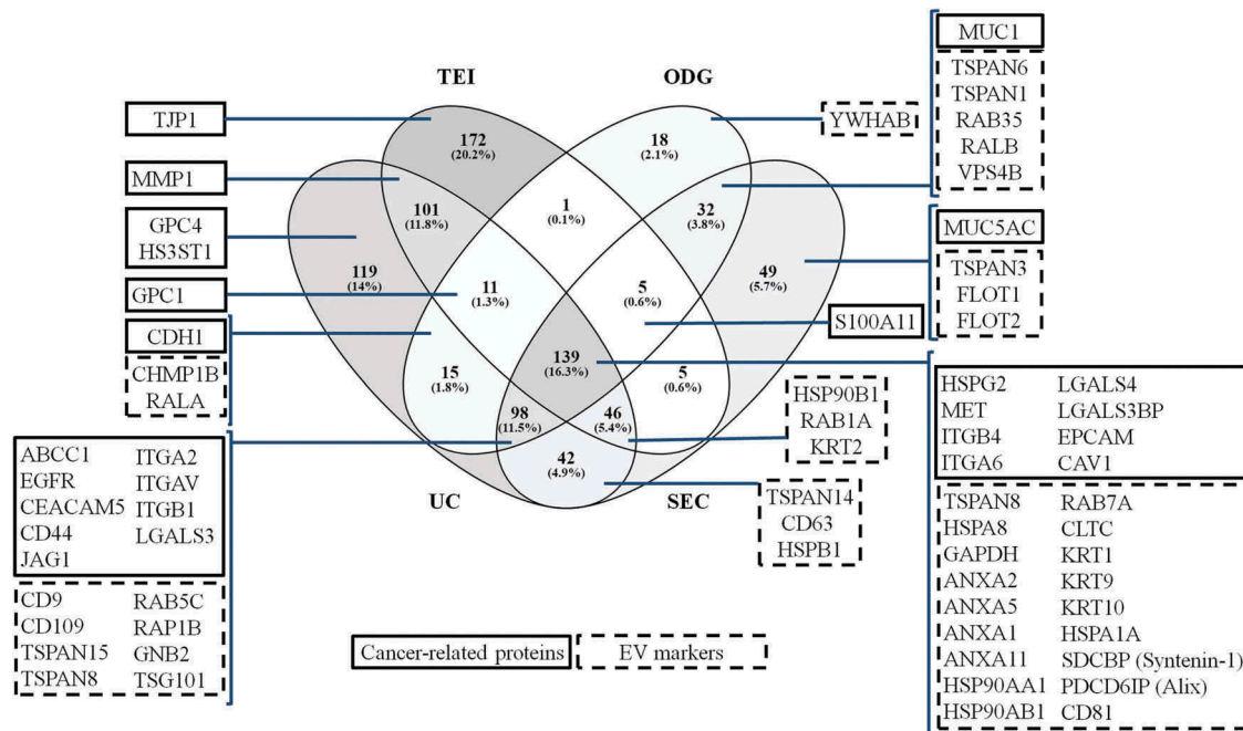
Figure 8. Representation of the proteins identified from extracellular vesicles (EVs) isolated by differential ultracentrifugation (UC), total exosome isolation (TEI), OptiPrep TM density gradient (ODG) and size exclusion chromatography (SEC) methodologies from glycoengineered MKN45 cells grown in the absence of FBS. Venn diagram demonstrates the number (and percentage) of unique and overlapping proteins identified by proteomic analysis for each EV isolation methodology. One experiment was conducted. Boxes highlight key cancer-related proteins (framed in full line) or EV markers (framed in dotted line) identified in the EV samples.
